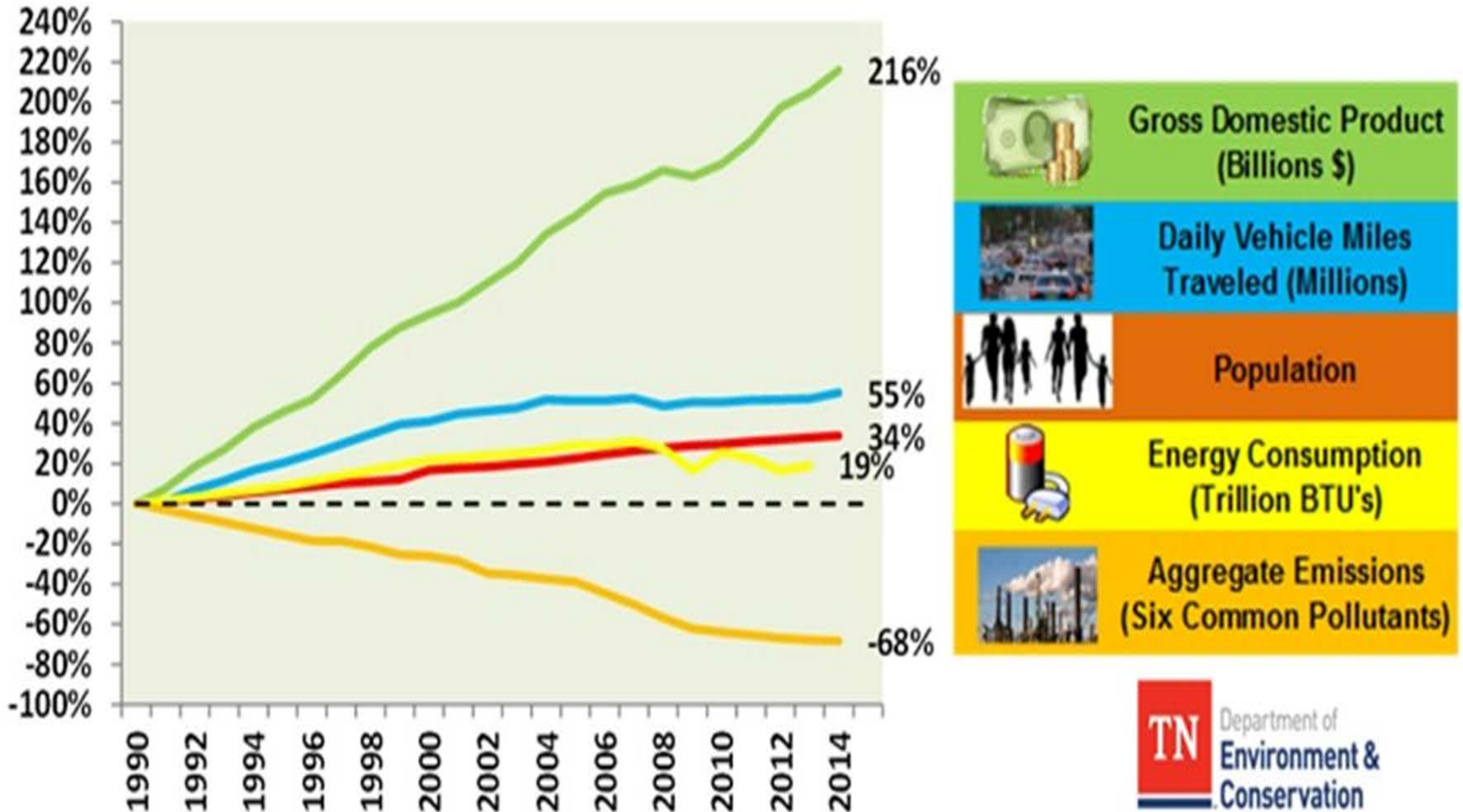
Tennessee Comparison of Growth Areas and Emissions 1990 to 2014
